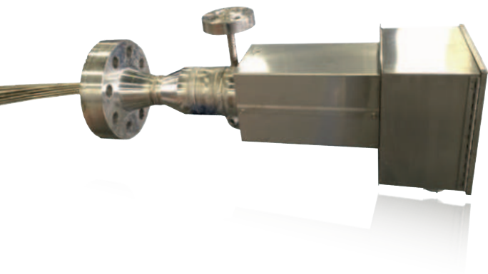
Multipoint thermometers for radial multipoint measurements in petrochemical processes
