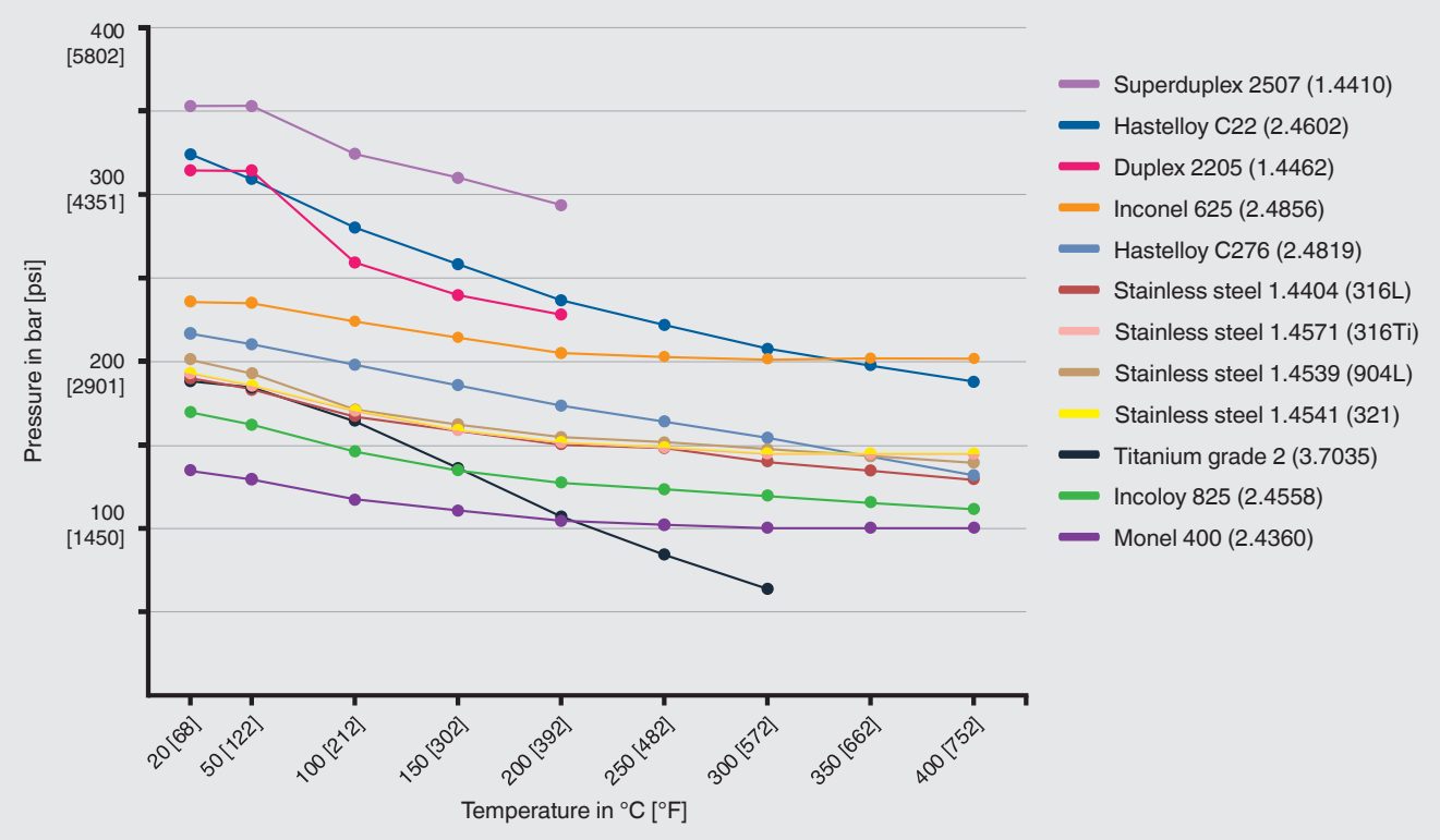
Pressure-temperature diagram Effective diameter of diaphragm Mb 52 mm
