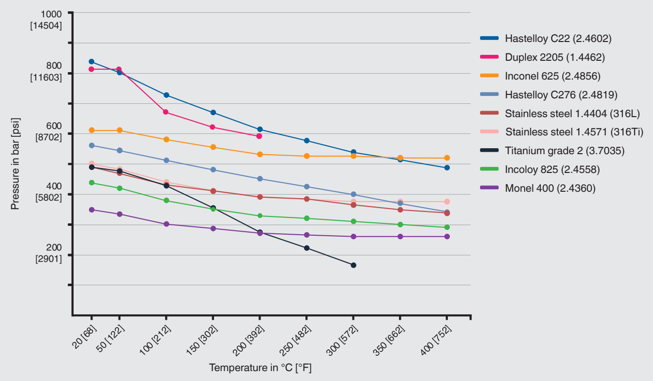
Pressure-temperature diagram Effective diameter of diaphragm Mb 29 mm
