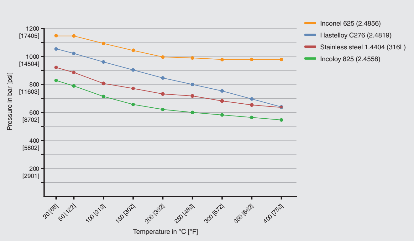
Pressure-temperature diagram Effective diameter of diaphragm Mb 22 mm
