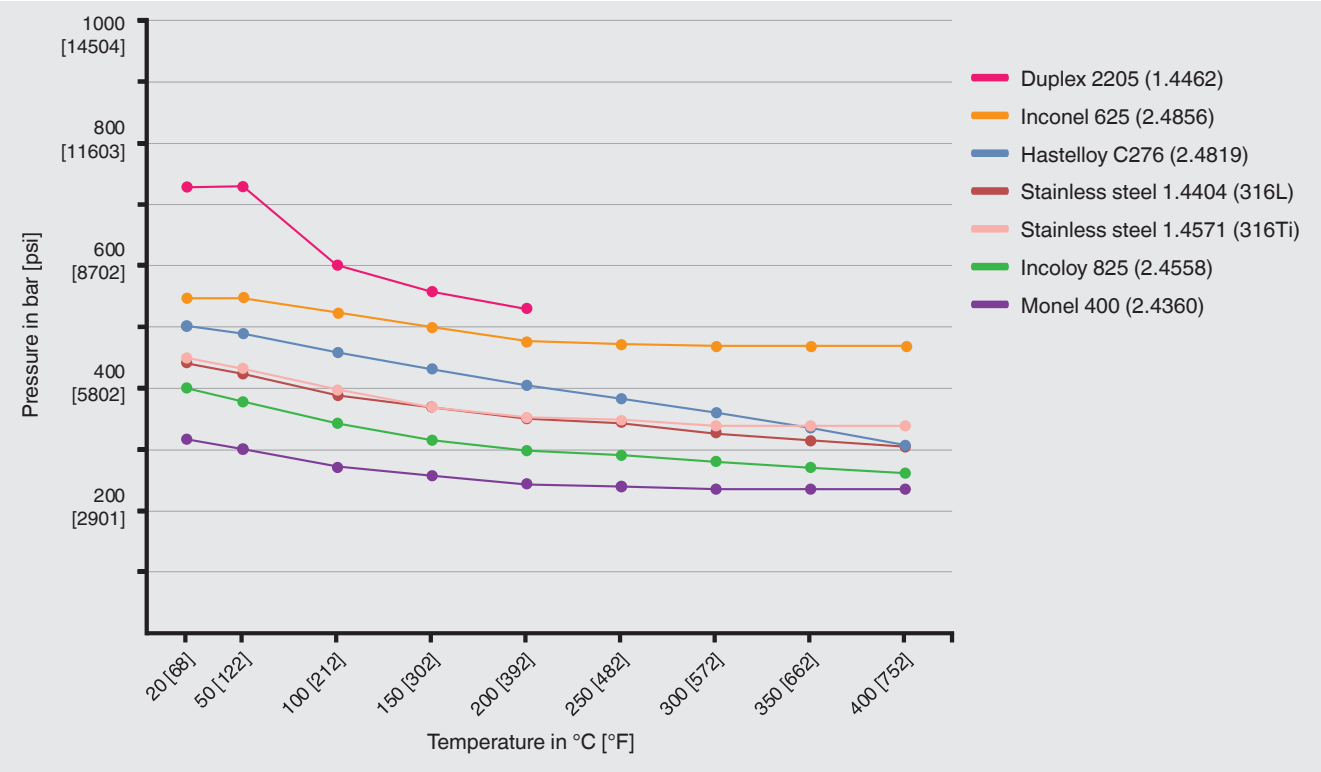
Pressure-temperature diagram Effective diameter of diaphragm Mb 40 mm
