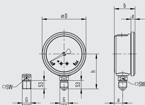
NS 50 [2"] and NS 63 [2 ½"], lower mount (radial)
